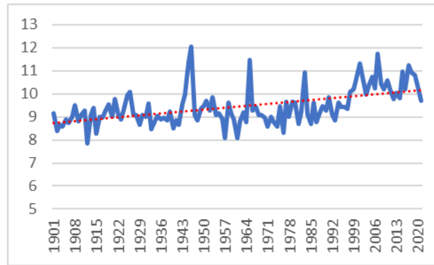
Fig. 2 Average air temperature of the vegetation period, C°
