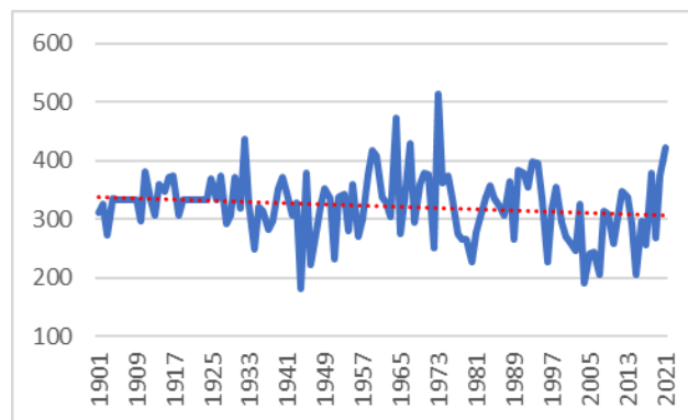
Fig. 3 Total rainfall during the vegetation period
